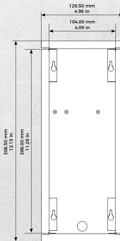
Mounting housing
