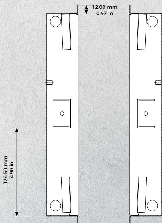
Mounting housing
