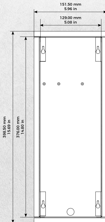
Mounting housing
