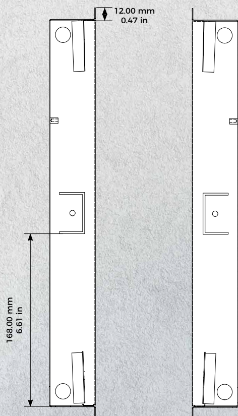
Mounting housing
